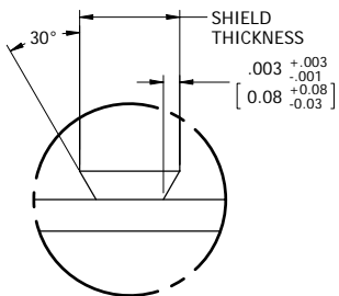
DETAIL A EDGE FINISH RECOMMENDATION
